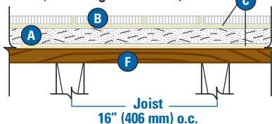
DensShield Tile Backer Over Conventional Joist (Exterior-glove Subfloor)
